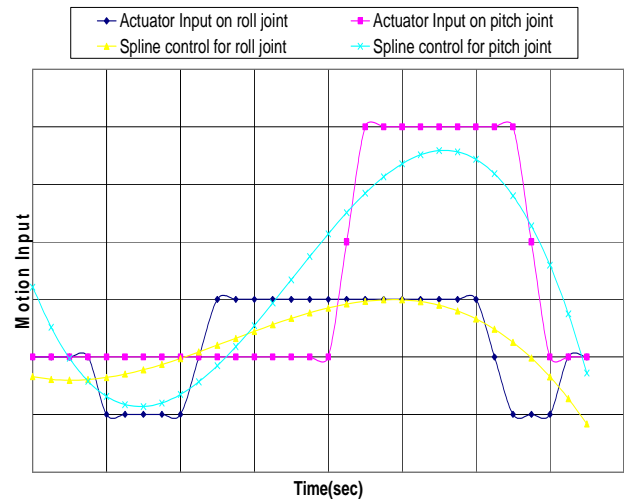
Figure 9. Trajectory of the hip joint
